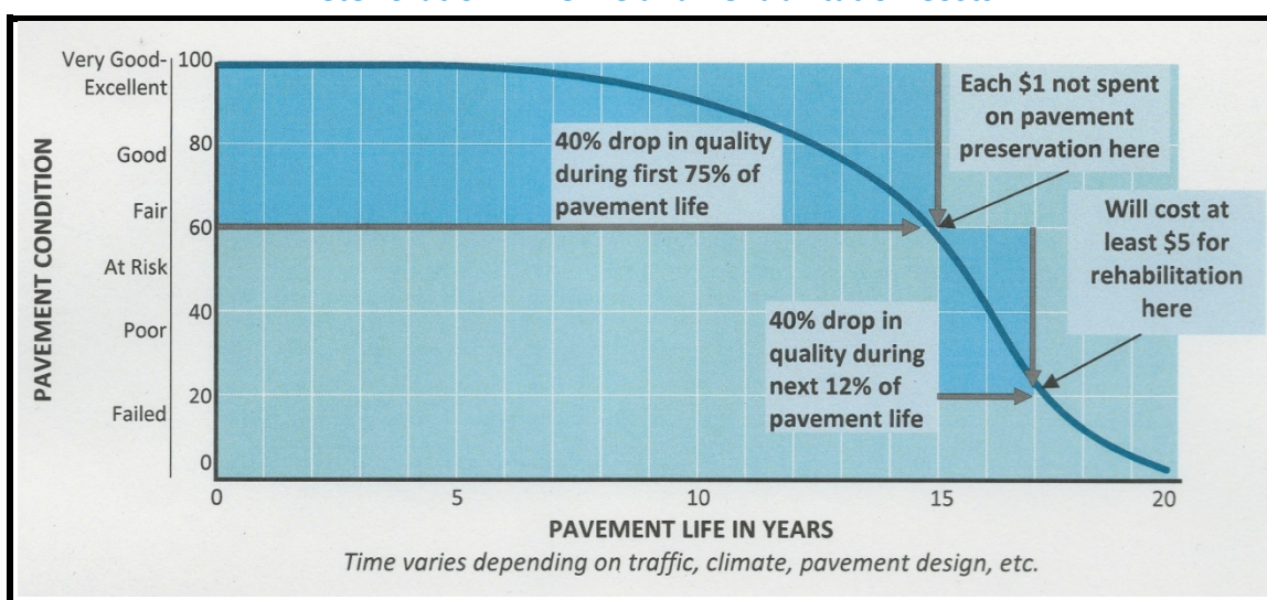
Pavement Life Cycle: Deterioration Timeline and Rehabilitation Costs
